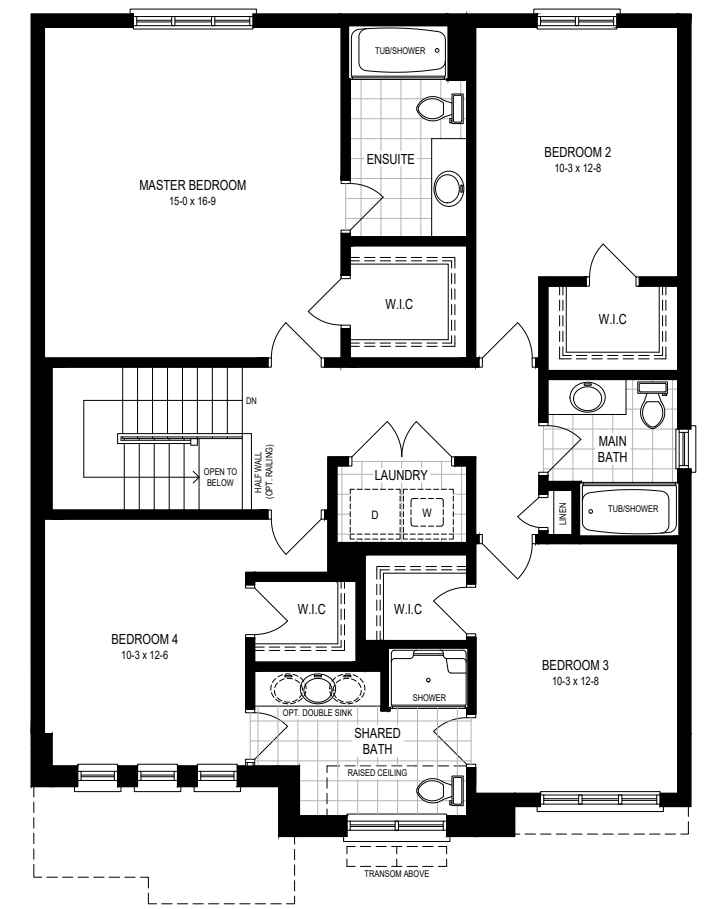
S2 - Second Floor
